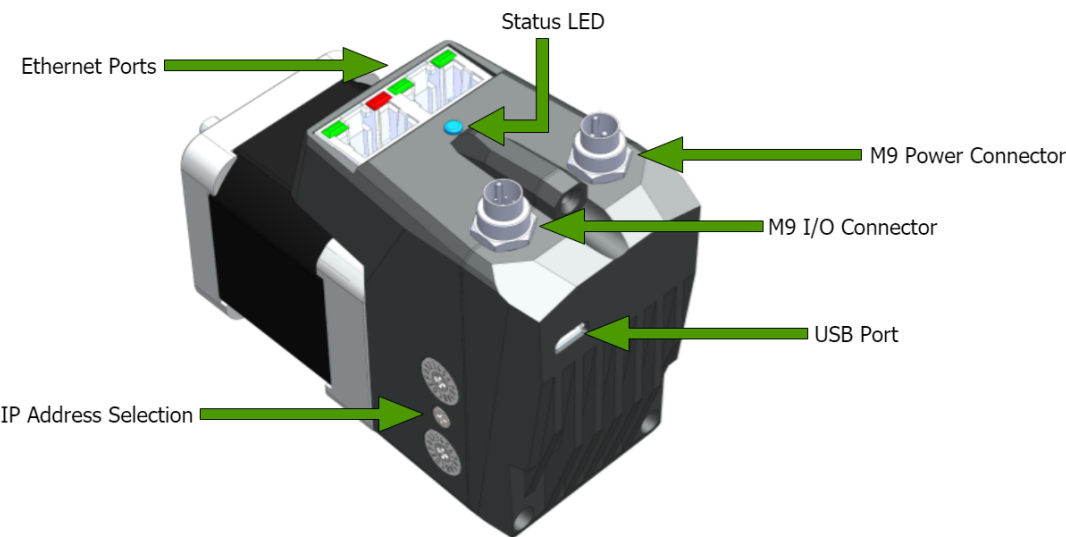
Figure: Overview of Connections and status LEDs
